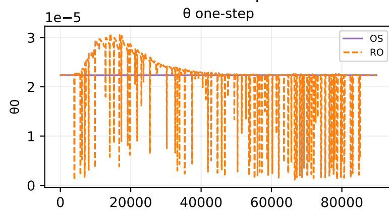
Oracle theta fit — sample 35
