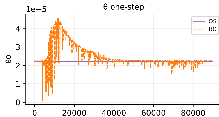
Oracle theta fit — sample 37
