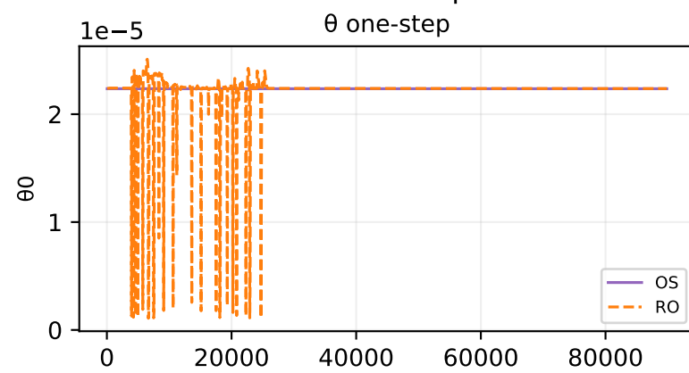
Oracle theta fit — sample 51
