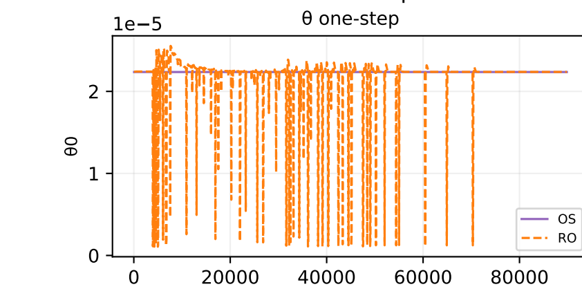
Oracle theta fit — sample 67
