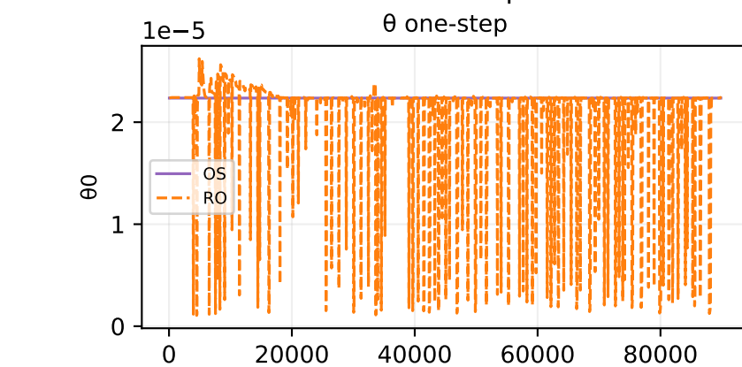
Oracle theta fit — sample 77
