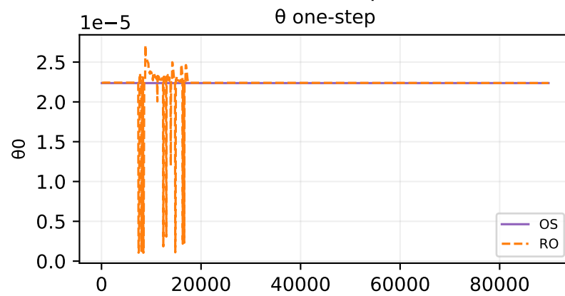
Oracle theta fit — sample 104
