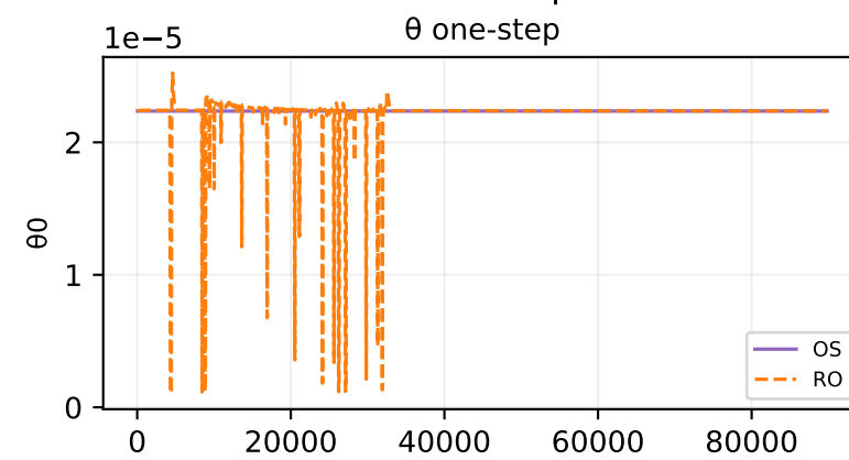
Oracle theta fit — sample 113
