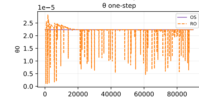
Oracle theta fit — sample 127
