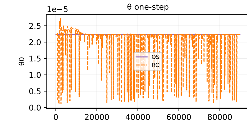
Oracle theta fit — sample 142
