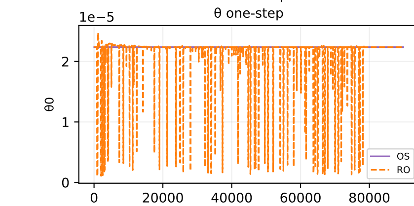
Oracle theta fit — sample 164
