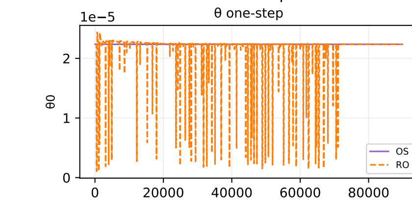
Oracle theta fit — sample 175
