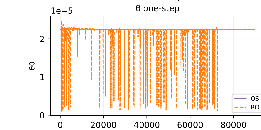
Oracle theta fit — sample 180
