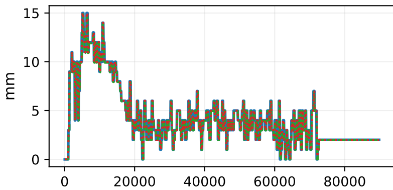
\theta_4
