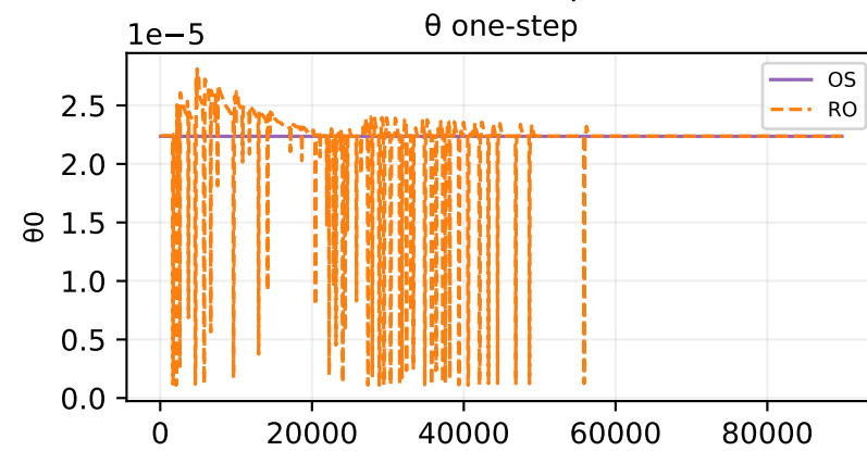
Oracle theta fit — sample 194
