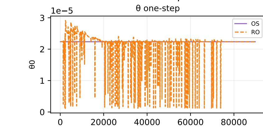
Oracle theta fit — sample 198
