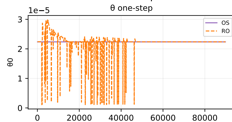
Oracle theta fit — sample 199
