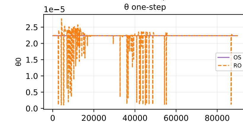
Oracle theta fit — sample 232
