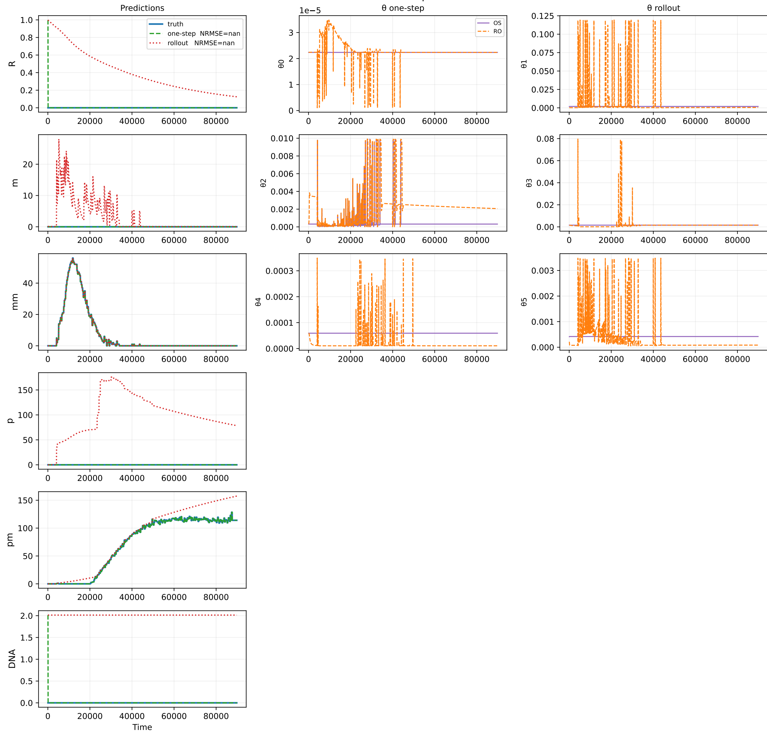
Oracle theta fit — sample 233
