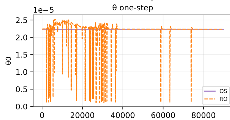
Oracle theta fit — sample 237
