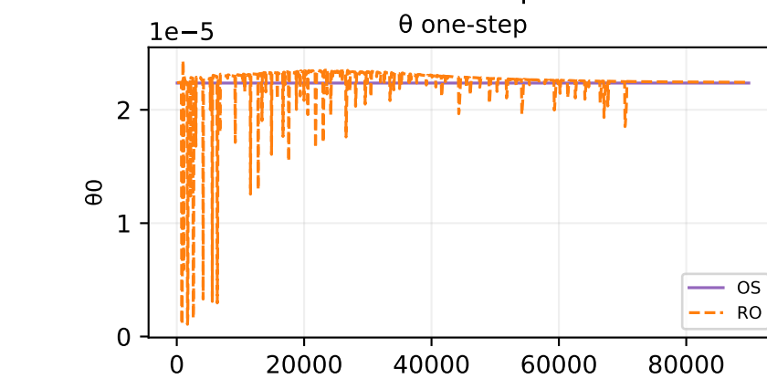
Oracle theta fit — sample 240
