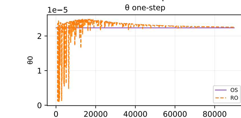
Oracle theta fit — sample 246
