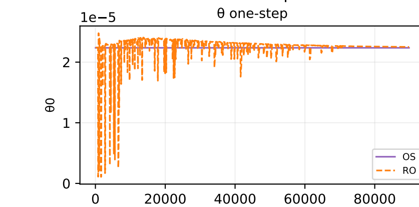
Oracle theta fit — sample 248
