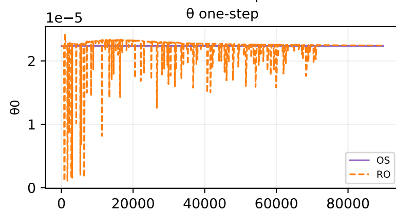
Oracle theta fit — sample 261
