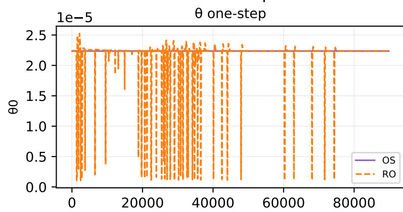
Oracle theta fit — sample 279
