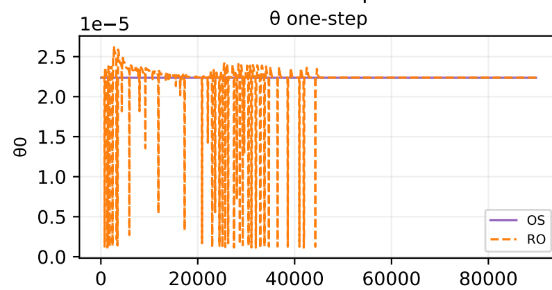
Oracle theta fit — sample 291
