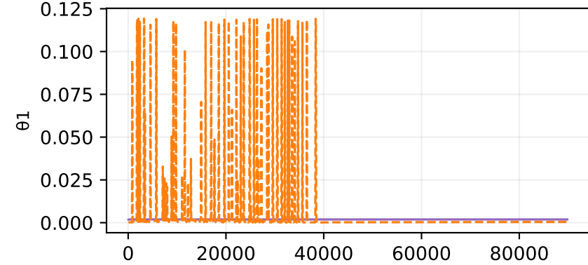
θ rollout
