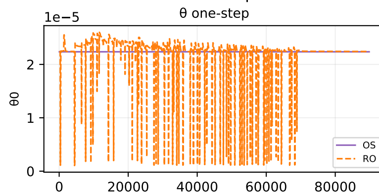
Oracle theta fit — sample 349
