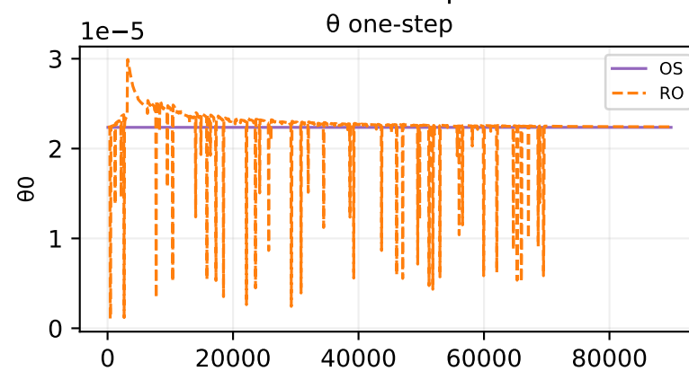
Oracle theta fit — sample 353
