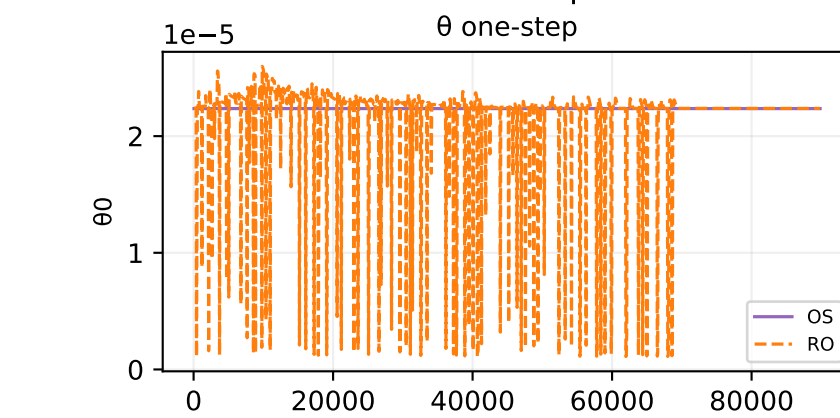
Oracle theta fit — sample 356
