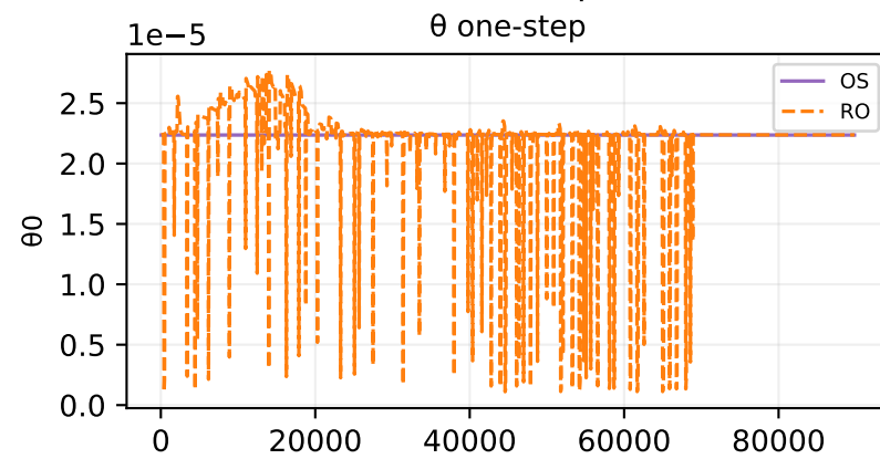
Oracle theta fit — sample 357
