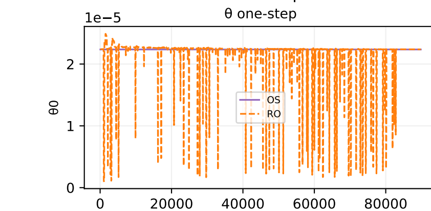
Oracle theta fit — sample 413
