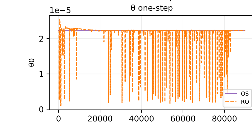
Oracle theta fit — sample 420
