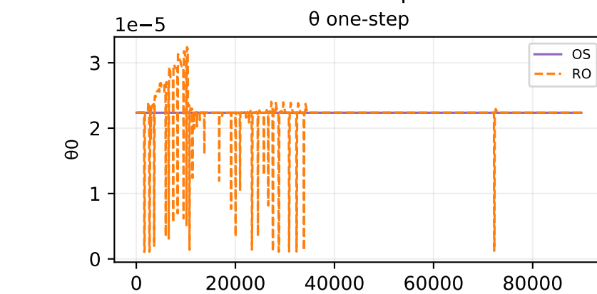
Oracle theta fit — sample 433
