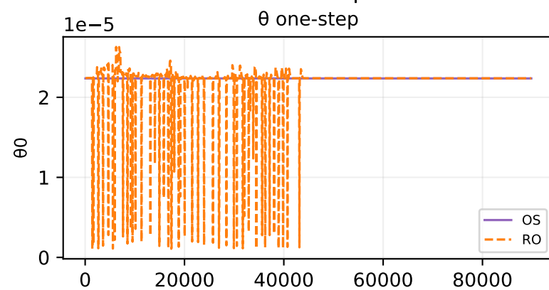
Oracle theta fit — sample 449
