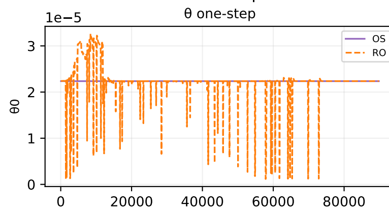
Oracle theta fit — sample 454
