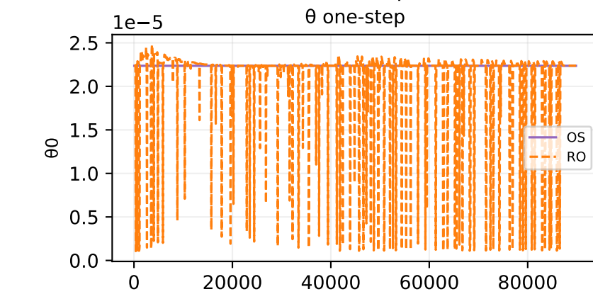
Oracle theta fit — sample 466
