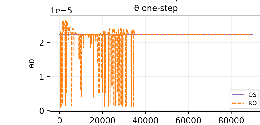
Oracle theta fit — sample 471
