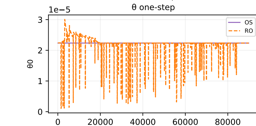
Oracle theta fit — sample 482
