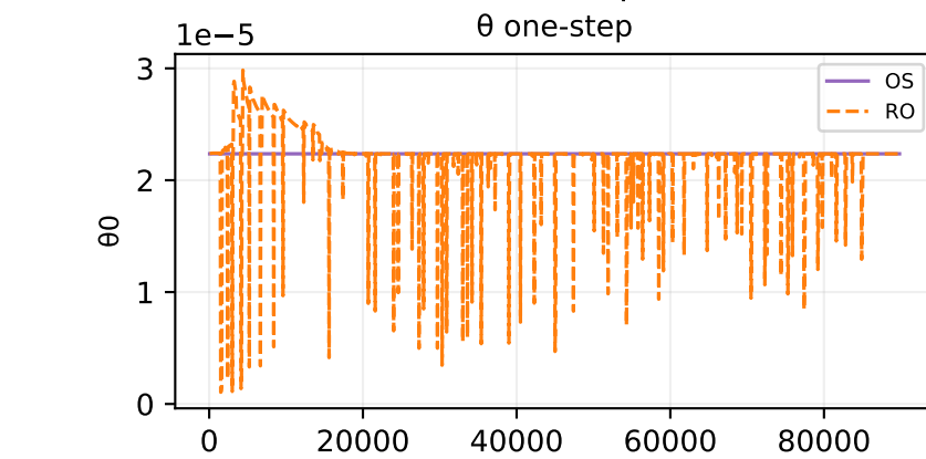
Oracle theta fit — sample 487
