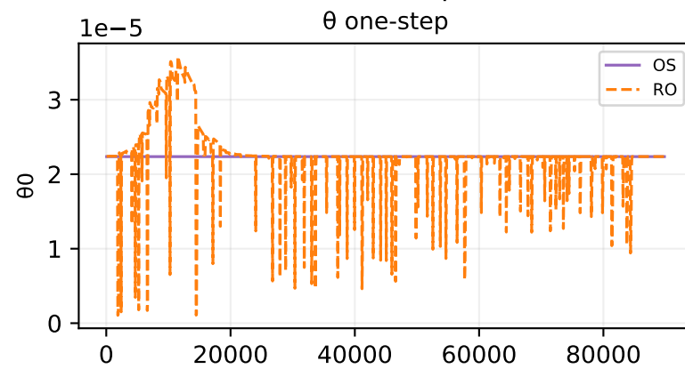
Oracle theta fit — sample 501
