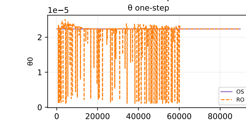
Oracle theta fit — sample 515
