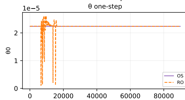
Oracle theta fit — sample 553
