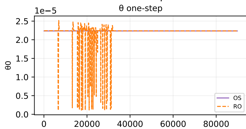
Oracle theta fit — sample 557
