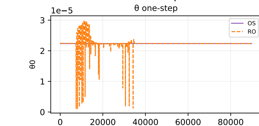
Oracle theta fit — sample 576
