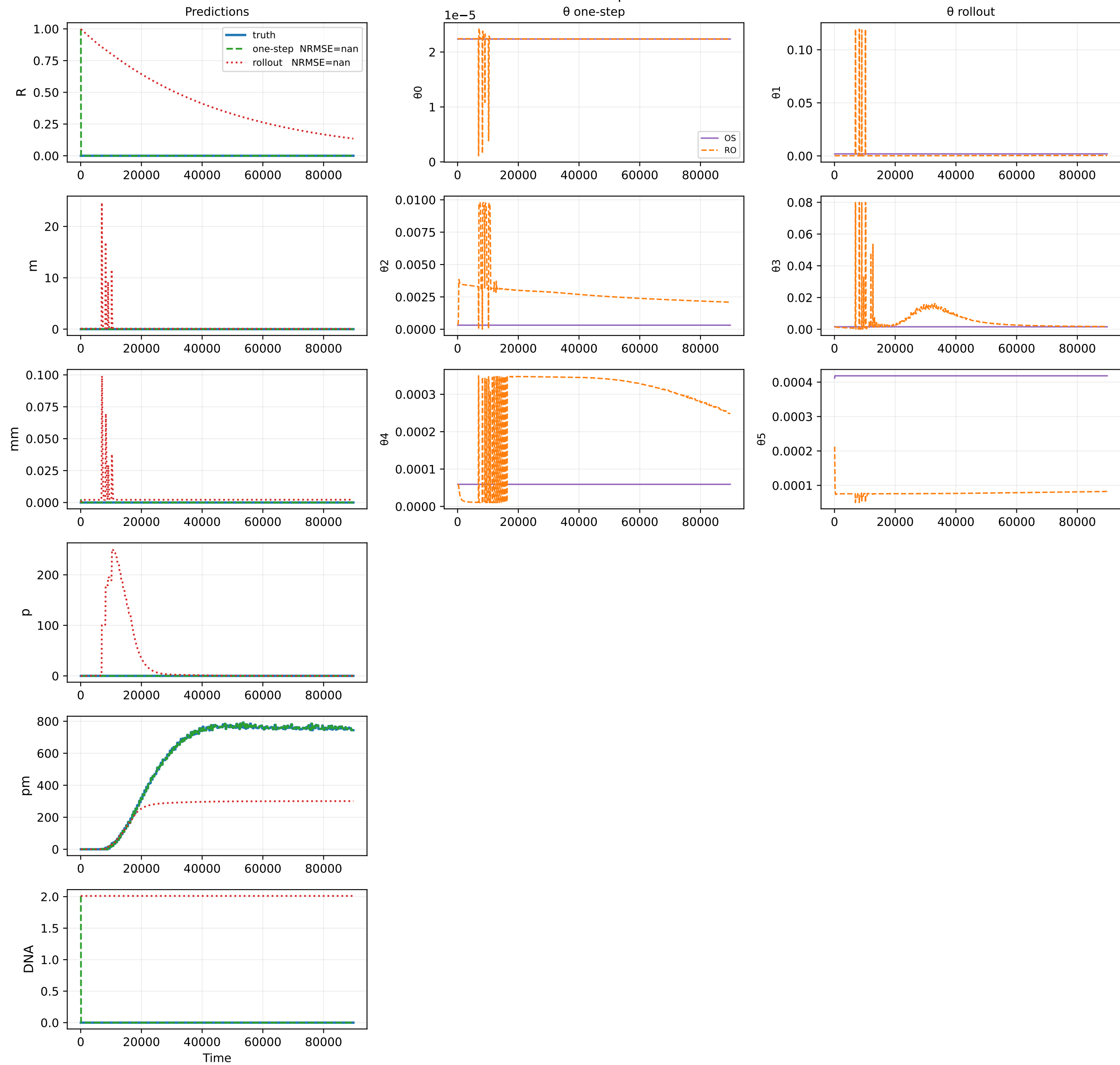
Oracle theta fit — sample 594
