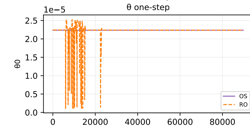
Oracle theta fit — sample 610
