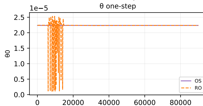
Oracle theta fit — sample 614
