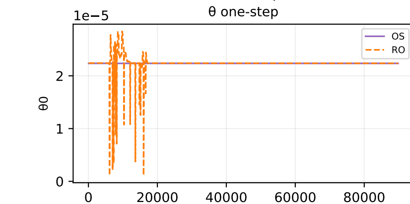
Oracle theta fit — sample 626
