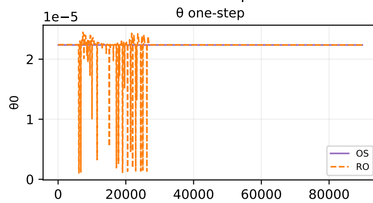
Oracle theta fit — sample 641
