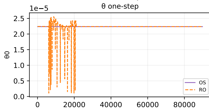
Oracle theta fit — sample 646
